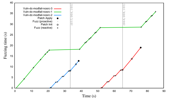
Figure 5. FUZZBUSTER discovers a new proactive vulnerability (green line) and begins refining it, then it receives two unexpected, reactive fault notifications from the host and addresses the reactive vulnerabilities (blue and red lines) before returning to its proactive fuzz-testing.
